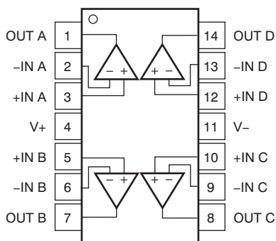
D Package: OPA1689 SOIC-14 Top View
